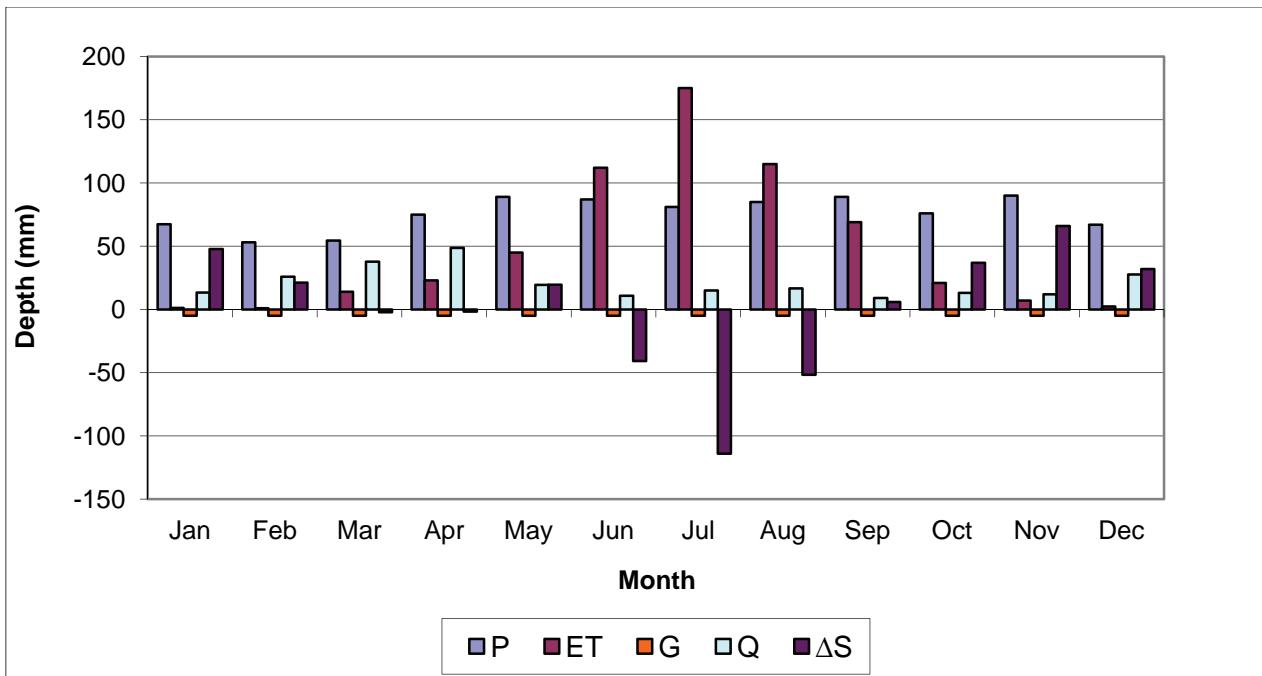
Figure 6.17: Monthly water budget components.
