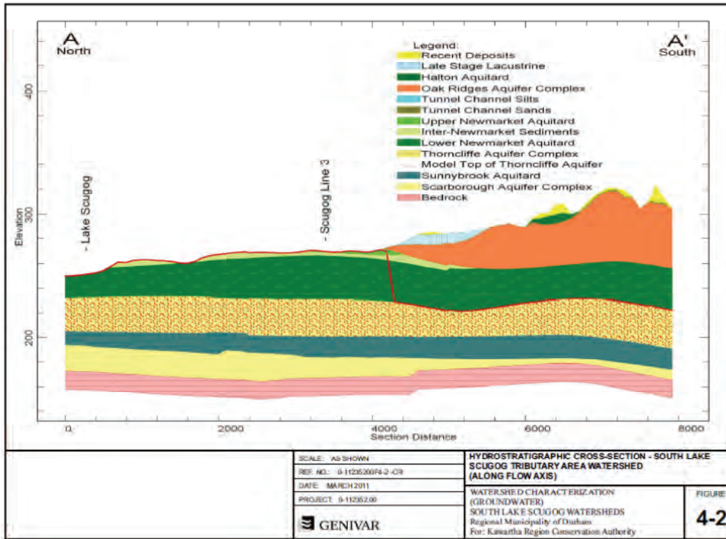
Figure 6.9: Crosssection A - A'.
