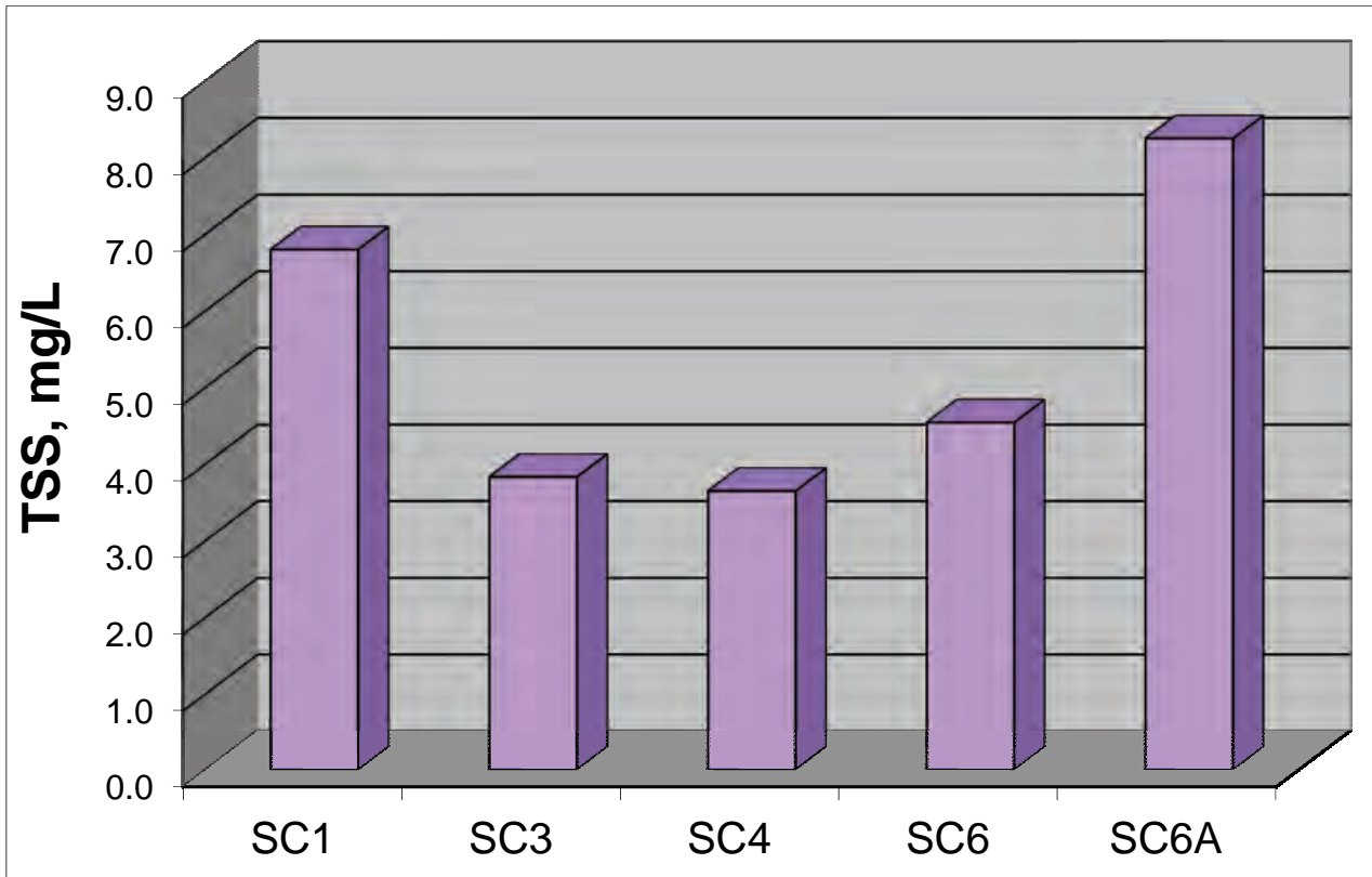
Figure 6.6: Average Total Suspended Solids concentrations from 2006 - 2010.
