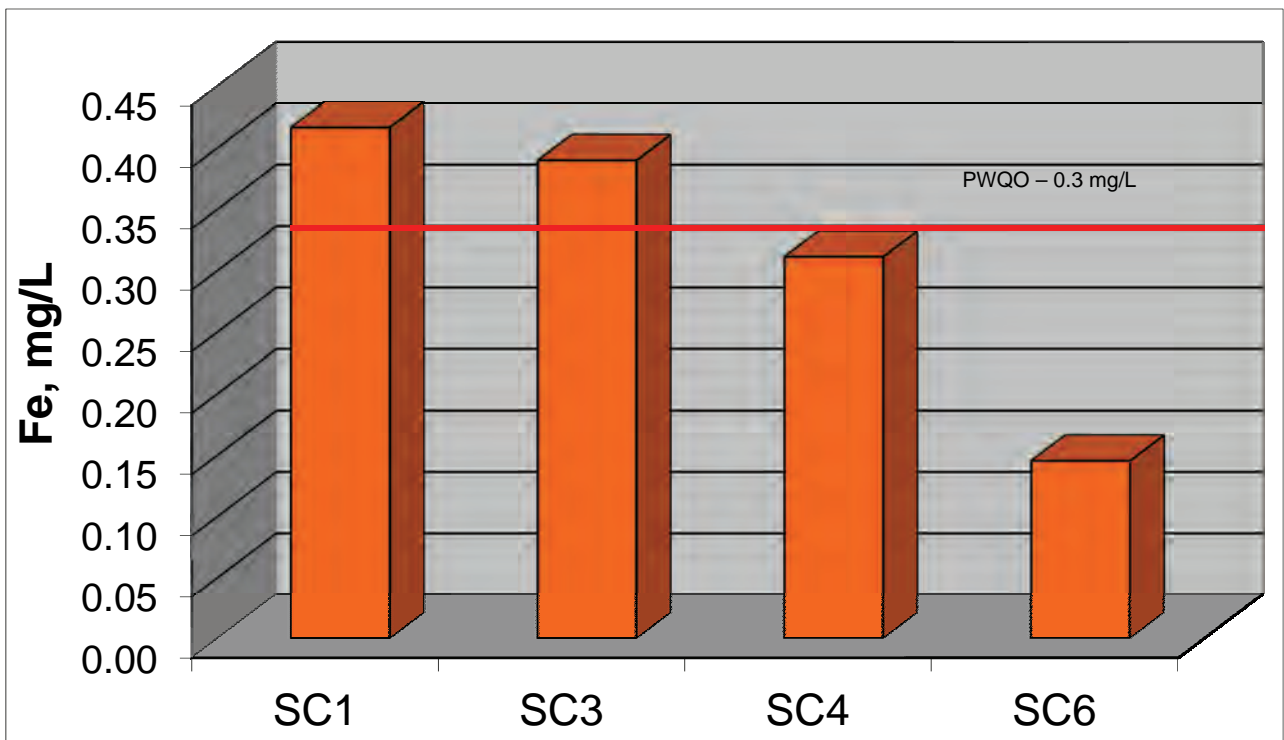
Figure 7.5: Average Iron concentrations from 2006 - 2010.
