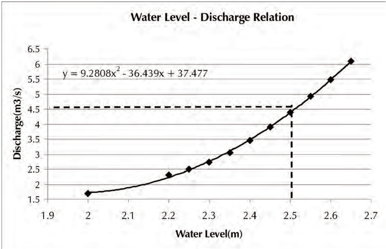
Figure 6.2: Sample rating curve.
