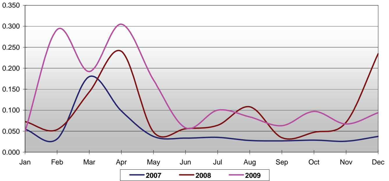
Figure 6.3: Monthly Discharge of Tributary 6 at Hwy 7A, 2007, 2008 and 2009.
