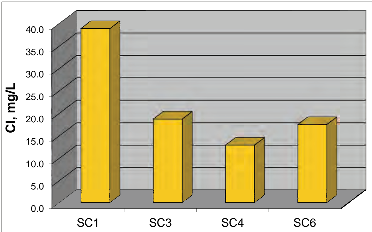
Figure 7.7: Average Chloride concentrations from 2006 - 2010.
