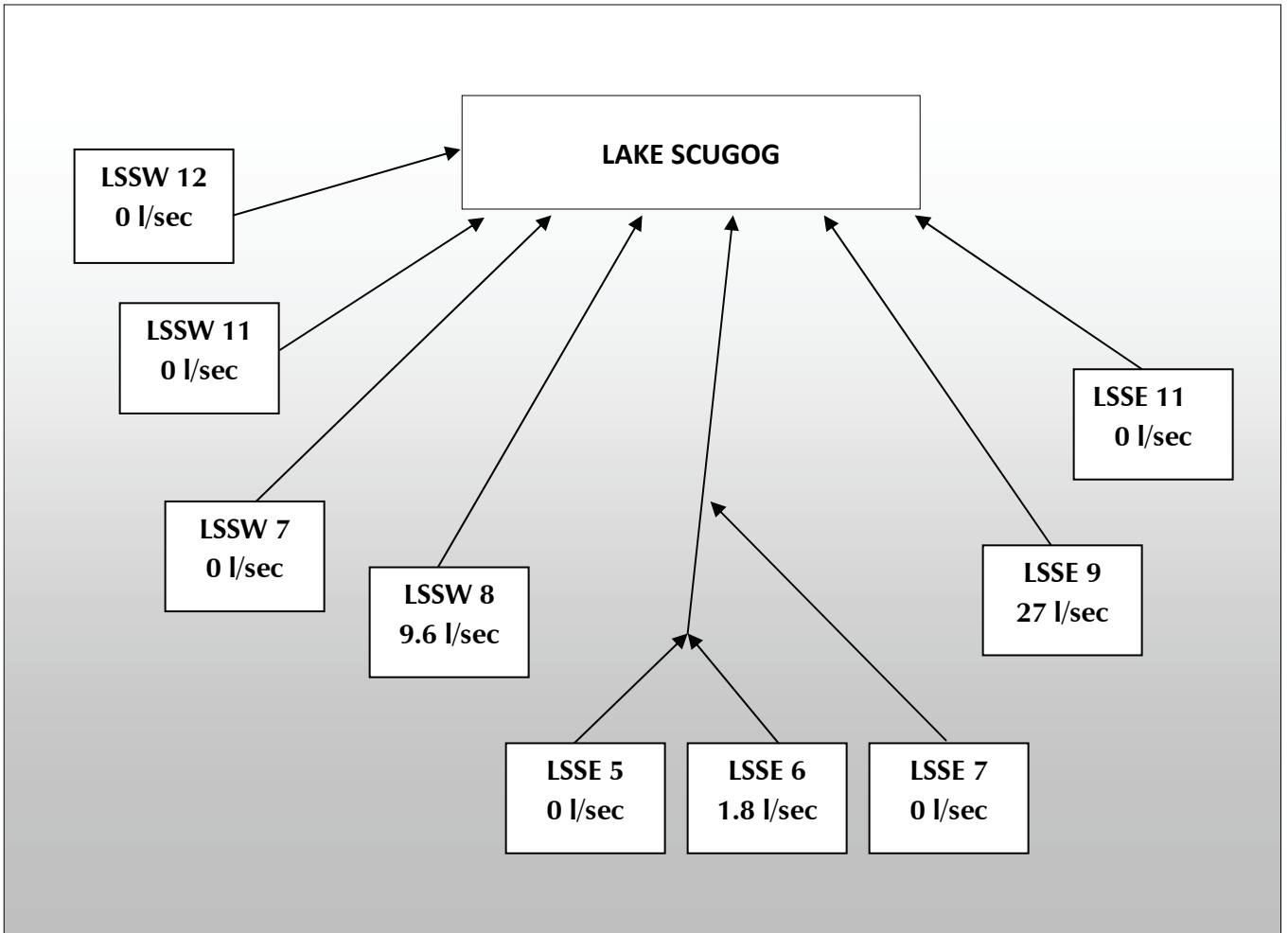
Figure 6.6: Baseflow monitoring diagram.
