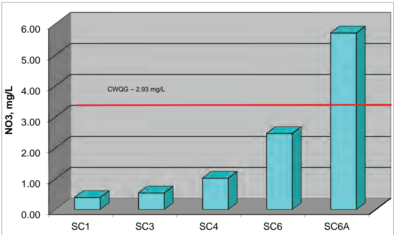
Figure 7.3: Average Nitrate concentrations from 2006 - 2010.
