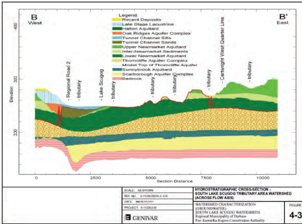
Figure 6.10: Crosssection B - B'.
