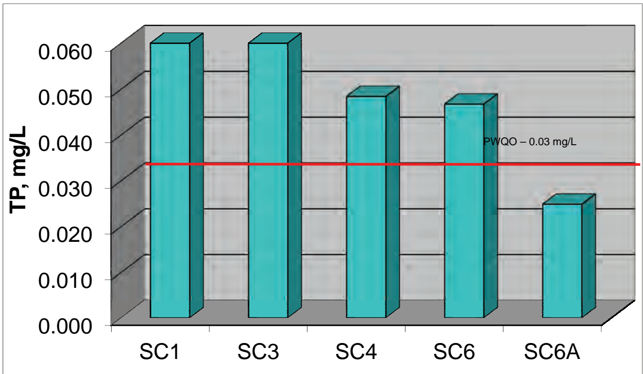
Figure 7.2: Average Phosphorus concentrations from 2006 – 2010.
