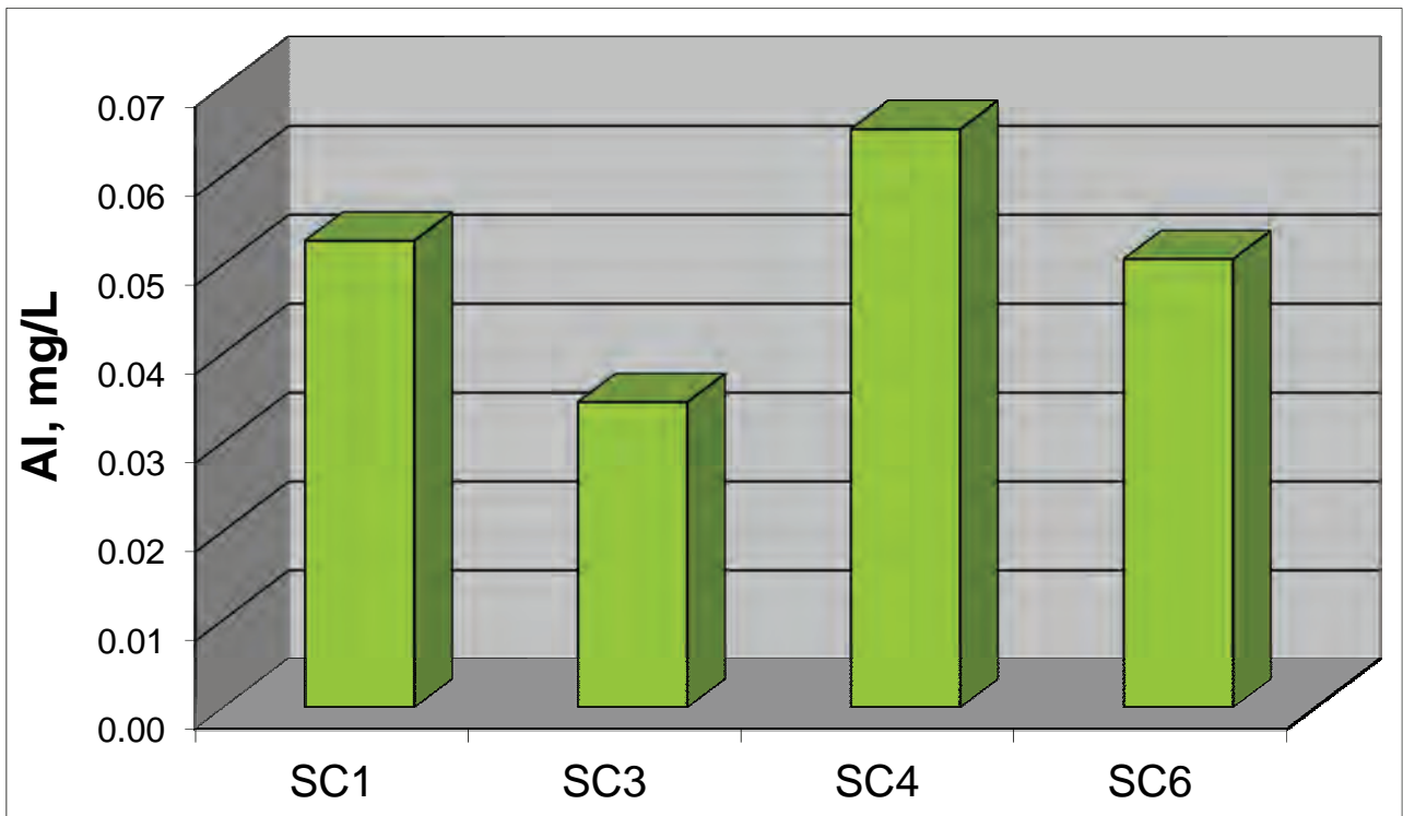
Figure 7.4: Average Aluminum concentrations from 2006 - 2010.
