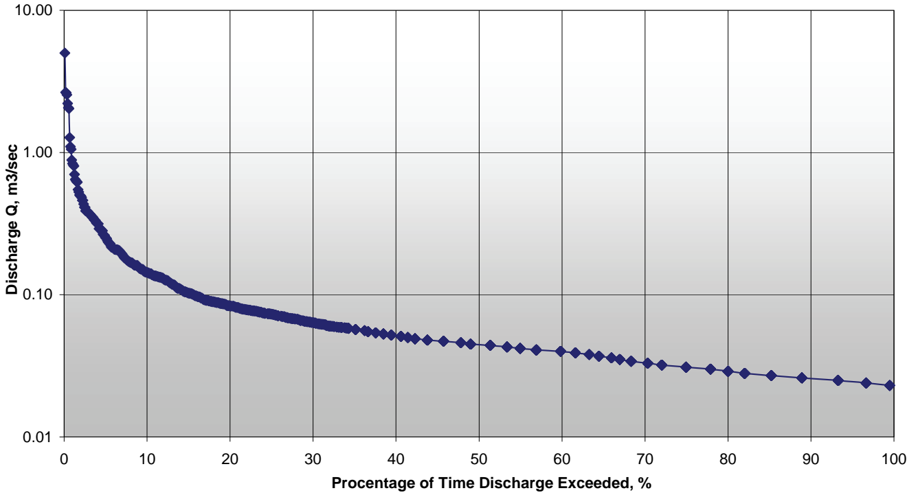
Figure 6.4: Semi-log plot of Flow Duration Curves, Tributary 6 at Hwy7A.
