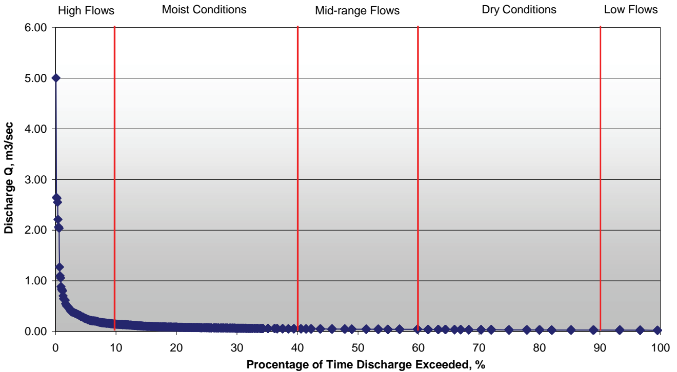
Figure 6.5: Flow Duration Curve, Tributary 6 at Hwy 7A.
